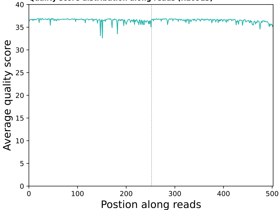
Quality score distribution along reads (R10913)
